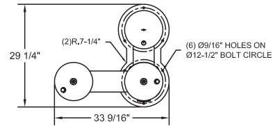
WODF-3FA-HC-PET & WODF-3FA-CHD-PET (REAR PET LOCATION)
