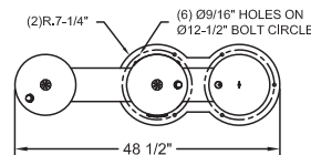
WODF-3FA-HC-PET & WODF-3FA-CHD-PET (SIDE PET LOCATION)
